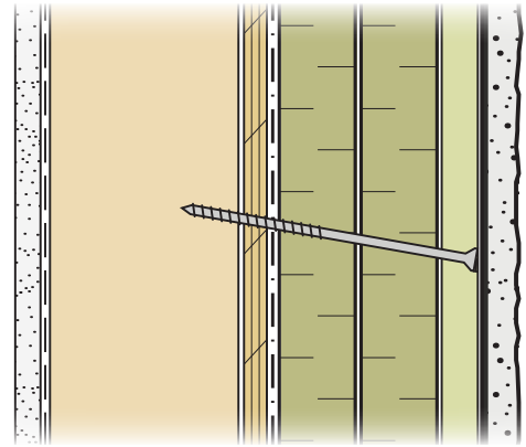
Screw at upward angle
