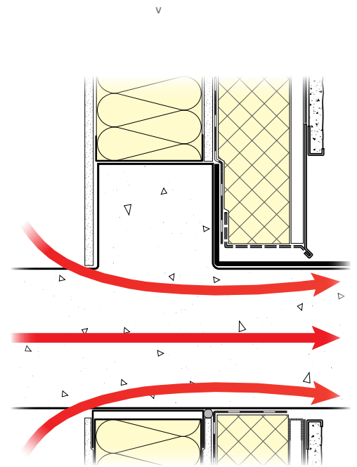
Balconies that penetrate the insulation can cause significant thermal bridging
