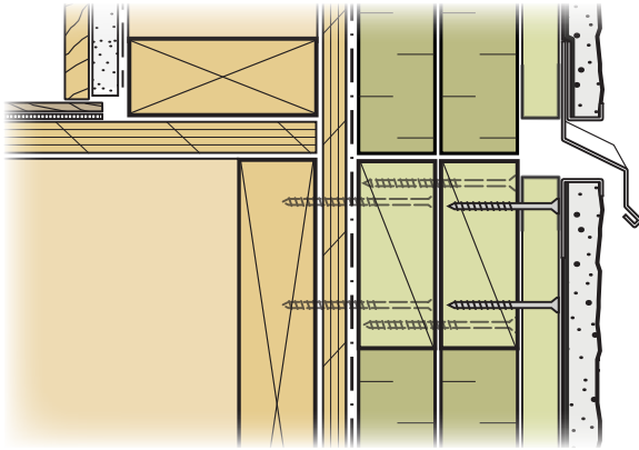
Deflection block
