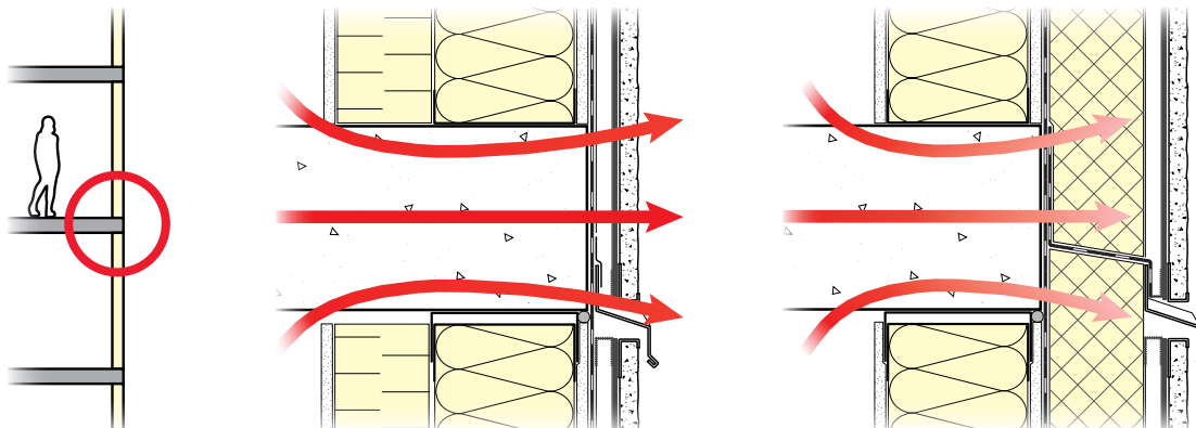
Exposed slab edges can result in significantly more thermal bridging compared to slab edges covered with insulation
