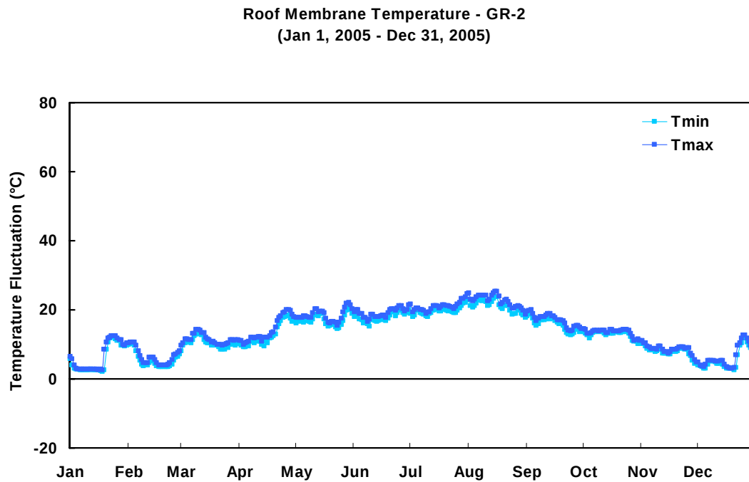
Figure 17 The daily maximum and minimum membrane temperatures measured on Green Roof 2.
