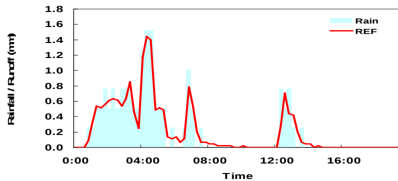
(a) Reference Roof REF
