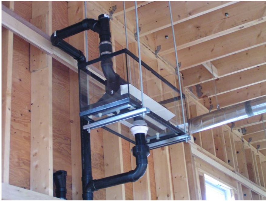
Photo 15 BCIT Green Roof Research Facility tipping bucket flow measurement system. Designed and built by the BCIT Technology Centre.
