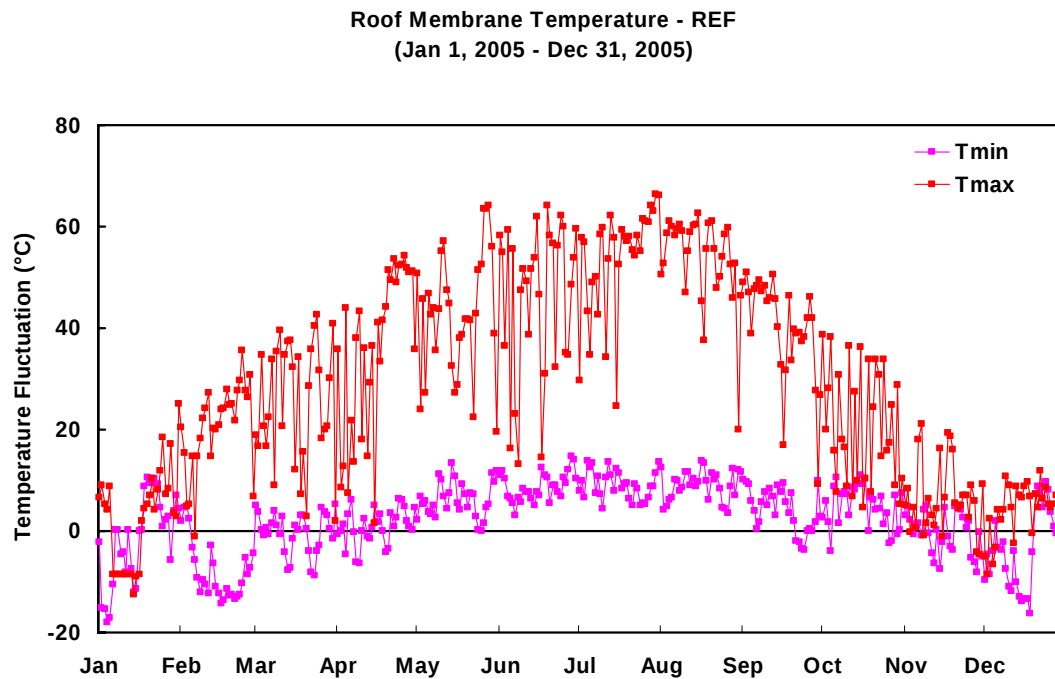
Figure 15 The daily maximum and minimum membrane temperatures measured on the Reference Roof.
