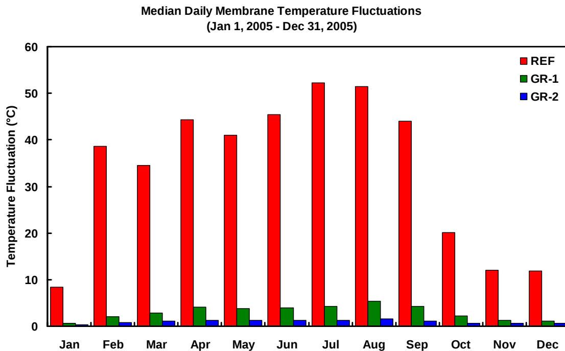
Figure 19 Median daily temperature fluctuation experienced by the roof membrane on the three roof sections at the BCIT Green Roof Research Facility (by month).
