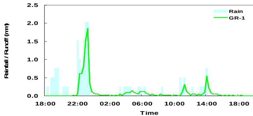
(b) Green Roof GR-1
