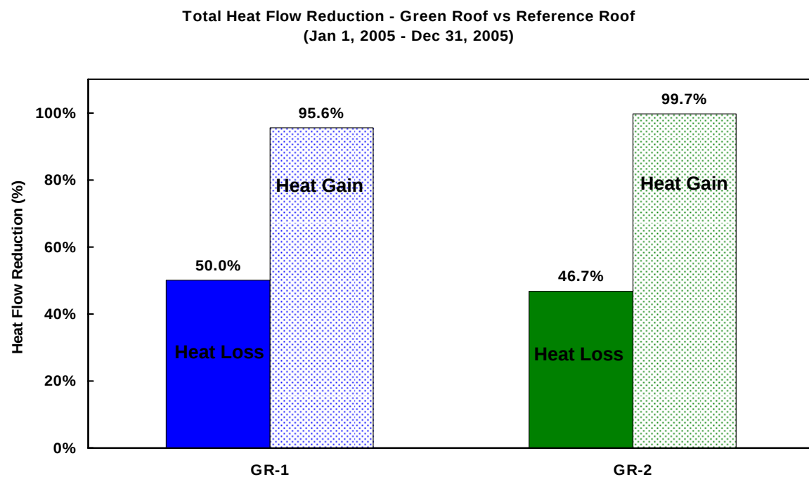
Figure 26 Heat flow reduction by the green roofs (GR-1 and GR-2) compared to the Reference Roof at the BCIT Green Roof Research Facility in 2005.
