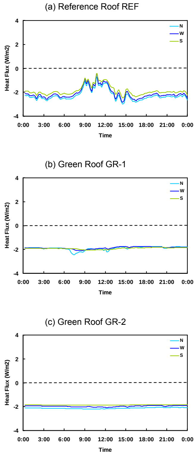
Figure 12 Heat flow through the three roof sections at the BCIT Green Roof Research Facility on a typical winter day (January 30, 2005). Each section contains three sensors – North (N), West (W) and South (S).
