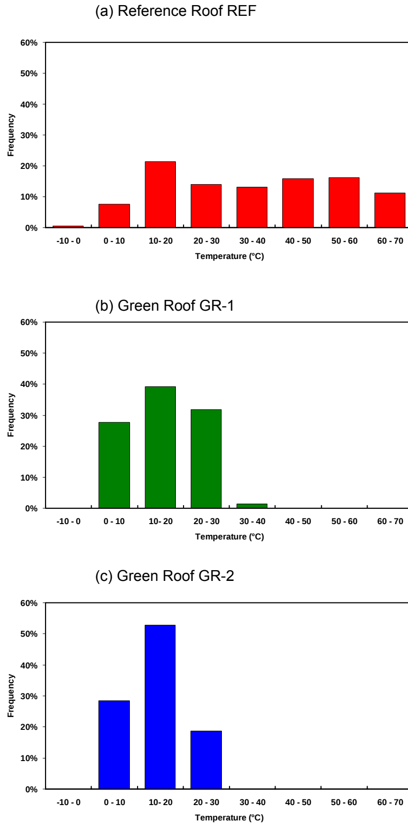
Figure 21 The maximum membrane temperature distribution of the three roof sections at the BCIT Green Roof Research Facility in 2005.
