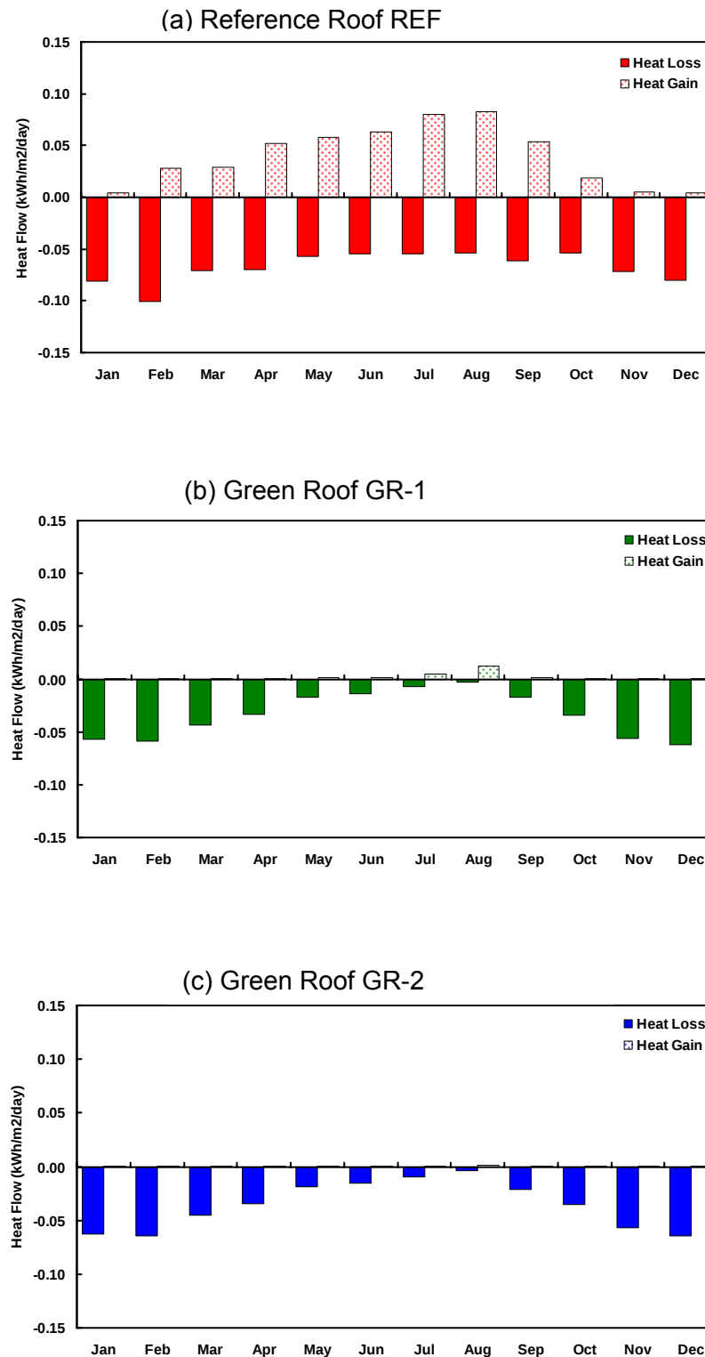
Figure 22 Average daily heat flow through the three roof sections at the BCIT Green Roof Research Facility (by month) in 2005.
