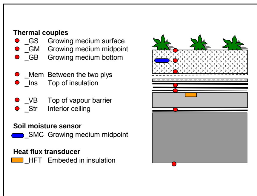
Figure 3 Cross-section of the BCIT Green Roof Research Facility's roofing system showing principal components and location of various sensors.
