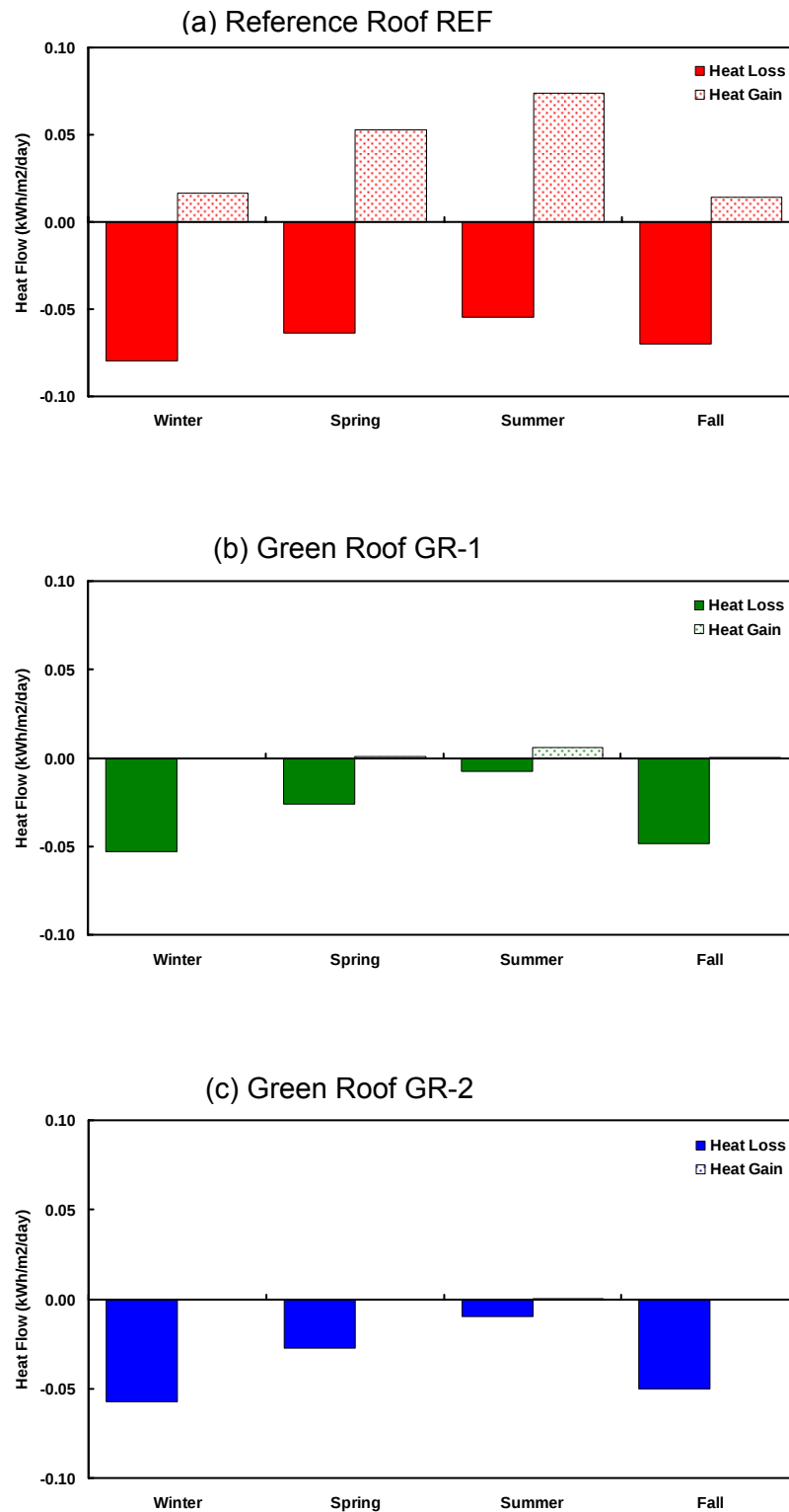
Figure 23 Average daily heat flow through the three roof sections at the BCIT Green Roof Research Facility (by season) in 2005.
