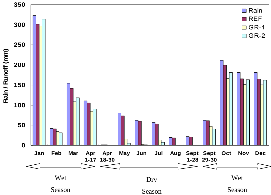
Figure 6 Rainfall and runoff comparison in the 2005 dry season and wet season.
