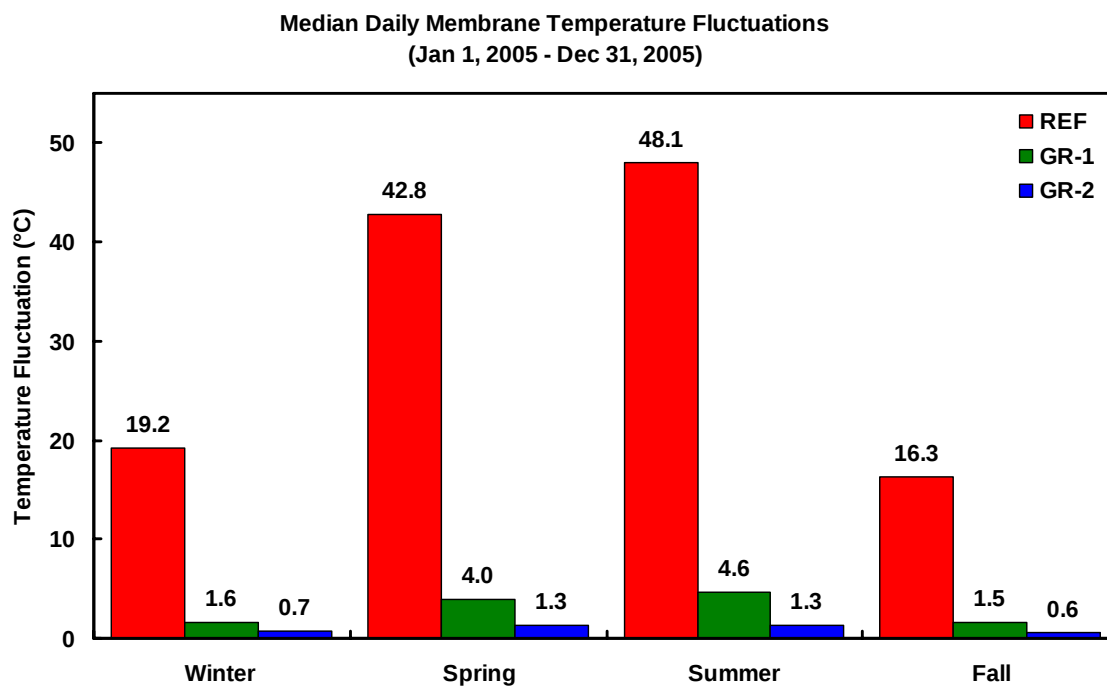
Figure 20 Median daily temperature fluctuation experienced by the roof membrane on the three roof sections at the BCIT Green Roof Research Facility (by season).
