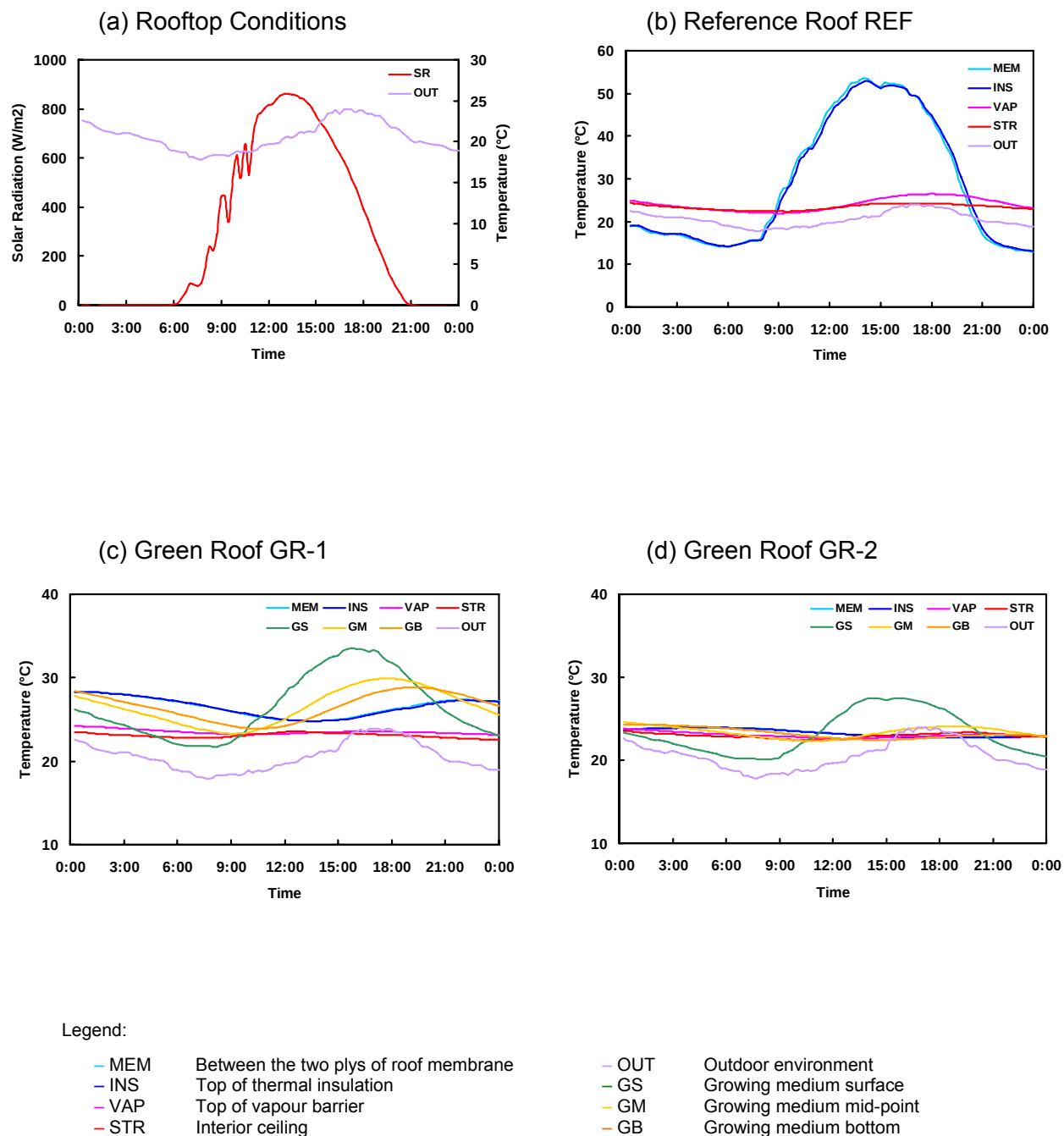
Figure 13 Weather conditions and temperature profile of the three roof sections at the BCIT Green Roof Research Facility on a typical summer day (August 1, 2005). Note that the temperature scale of the green roof plots was expanded for clarity. Refer to Figure 3 for instrumentation location symbols.
