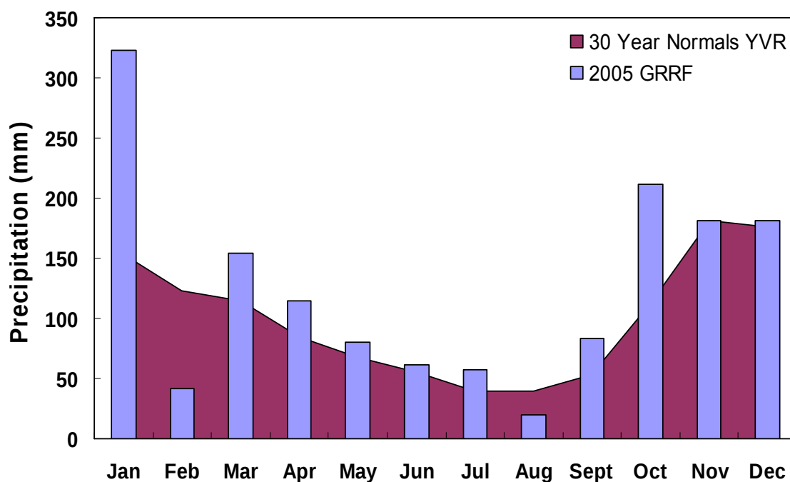
Figure 4 Precipitation at the BCIT Green Roof Research Facility compared to 30 year normals at the Vancouver International Airport.
