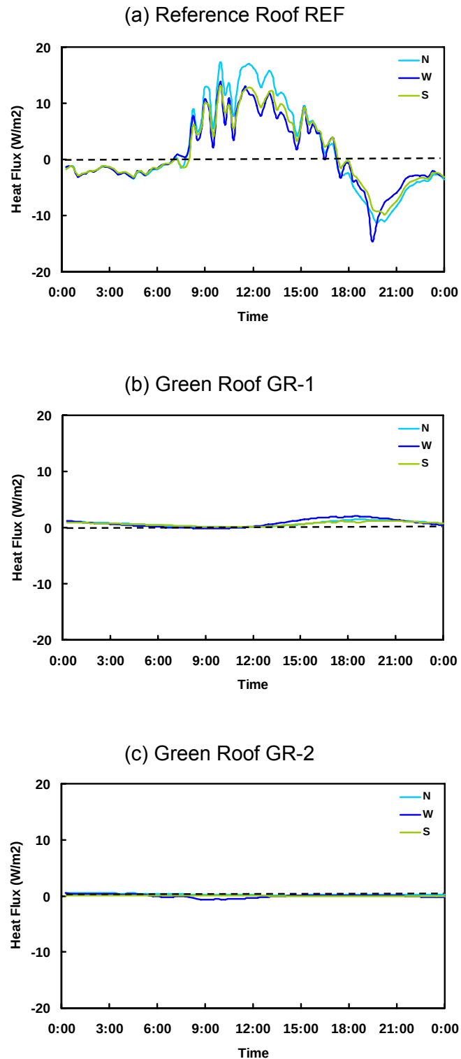
Figure 14 Heat flow through the three roof sections at the BCIT Green Roof Research Facility on a typical summer day (August 1, 2005). Each section contains three sensors – North (N), West (W) and South (S).
