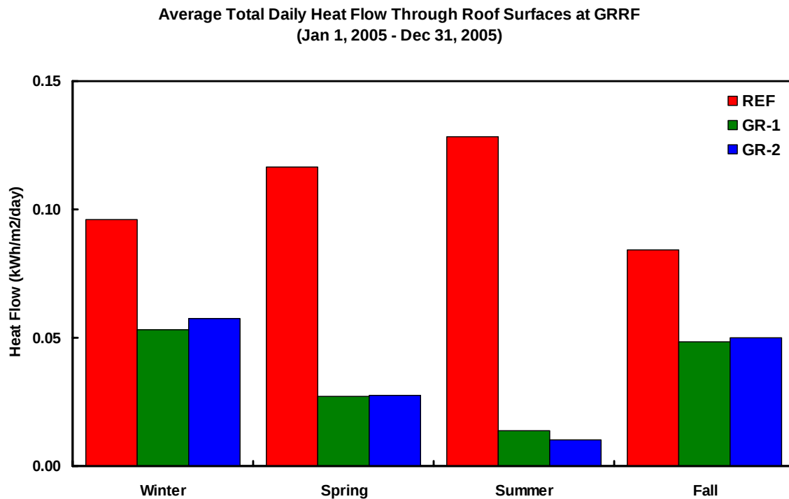
Figure 24 Average daily energy demand due to heat flow through the roof for the three roof sections in 2005 (a) by month and (b) by season.
