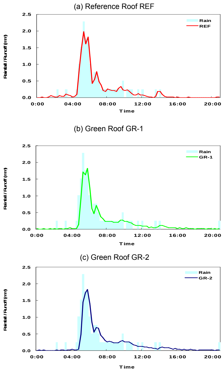
Figure 10 Reference roof and green roof runoff comparison during the November 1–2 rain event. 17.5 mm of rainfall were recorded over 11 hours and 45 minutes.
