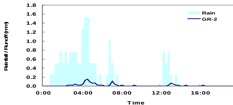
(c) Green Roof GR-2
