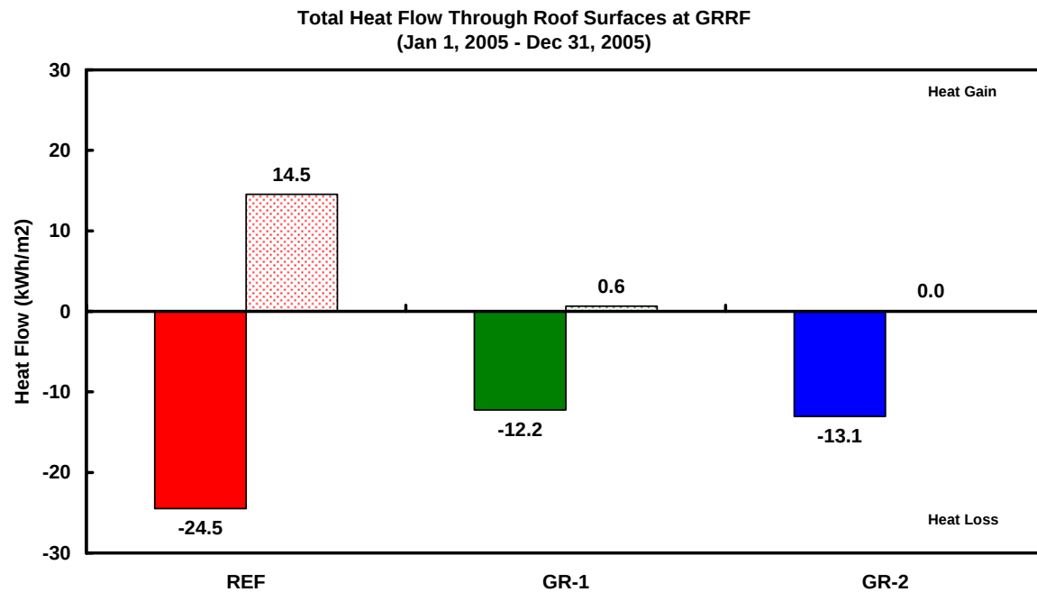
Figure 25 Annual energy demand due to heat flow through the roof for the three roof sections at the BCIT Green Roof Research Facility in 2005.
