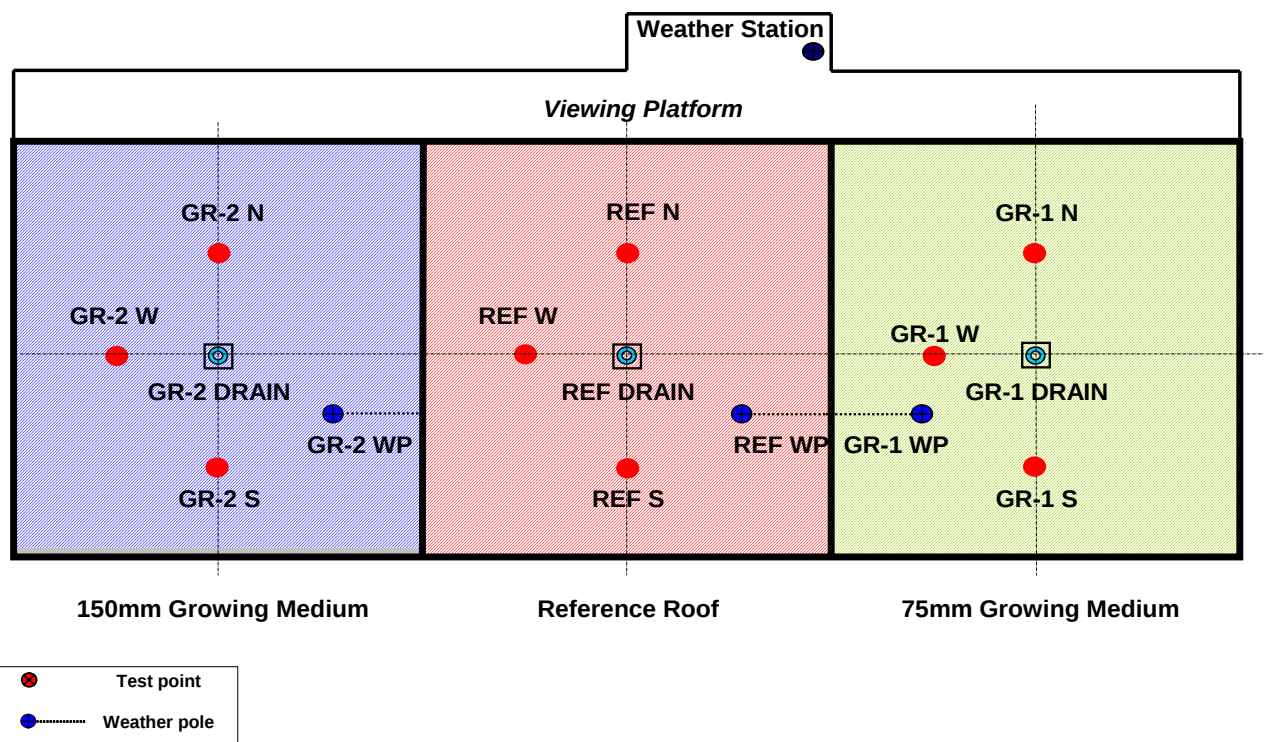
Figure 2 Schematic roof plan of the BCIT Green Roof Research Facility showing instrumentation locations and locations of weather poles and weather station.
