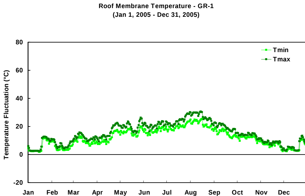
Figure 16 The daily maximum and minimum membrane temperatures measured on Green Roof 1.
